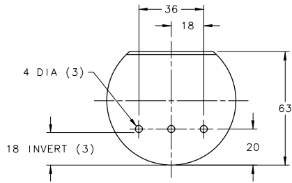
BAFFLE DETAIL
